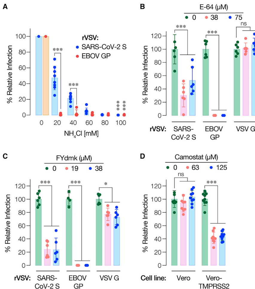
Figure 2. rVSV-SARS-CoV-2 S Infection Requires the Activity of Cysteine Cathepsin Proteases
