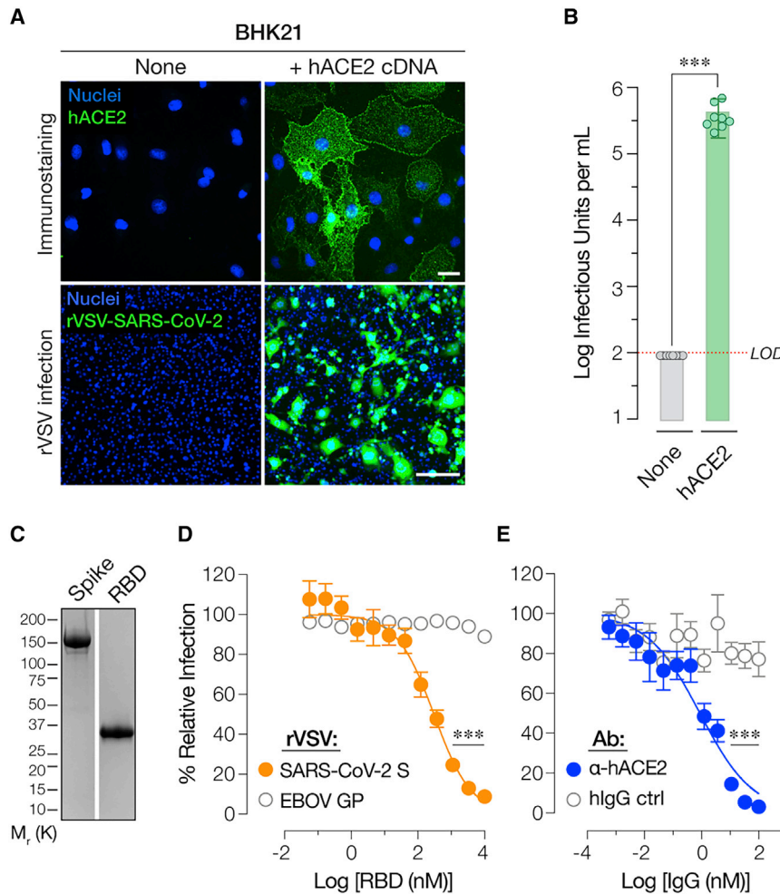
Figure 3. rVSV-SARS-CoV-2 S Infection Requires Human ACE2
